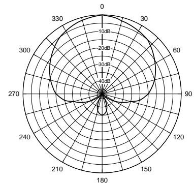
Vertical Pattern
