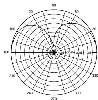
Vertical Pattern
